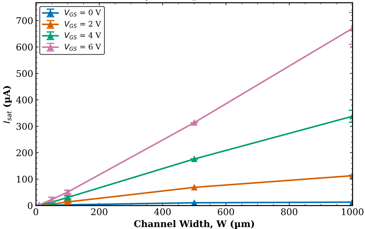
All Chips - Combined I_{sat} vs W | L = 8\text{ }\mu\text{m} (mean \pm std)
